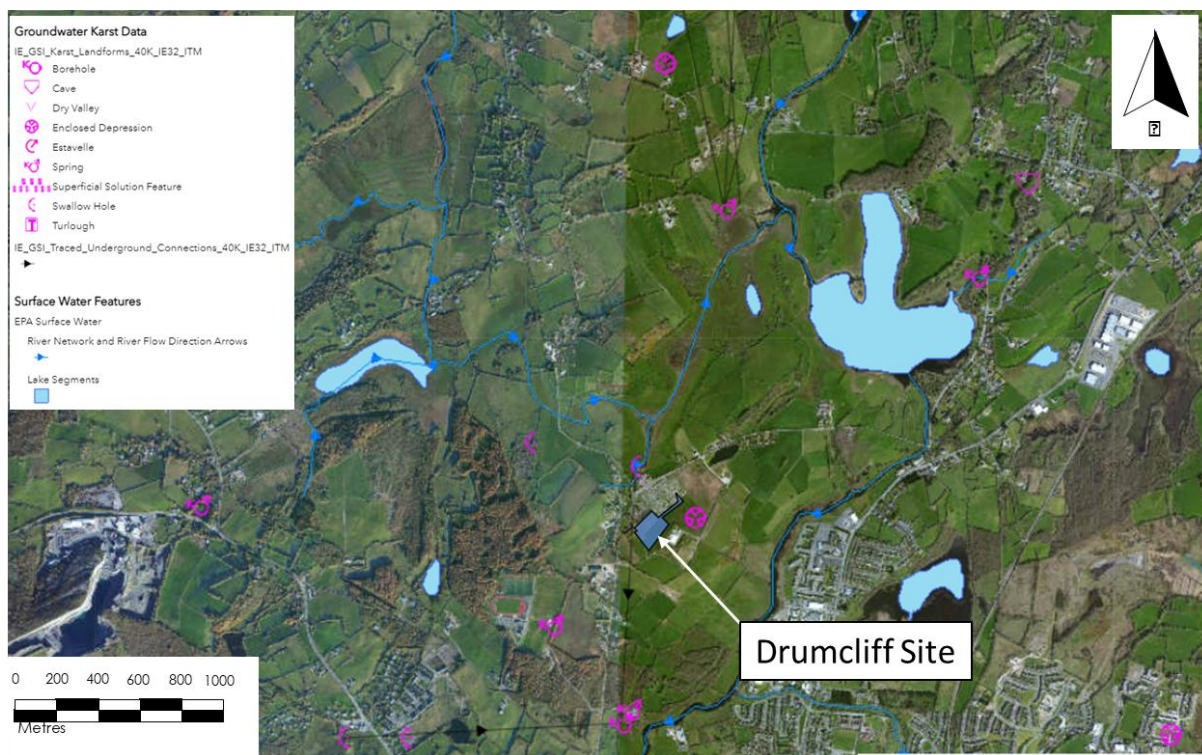
Figure B: Local Surface Watercourses with Mapped Karst Features
