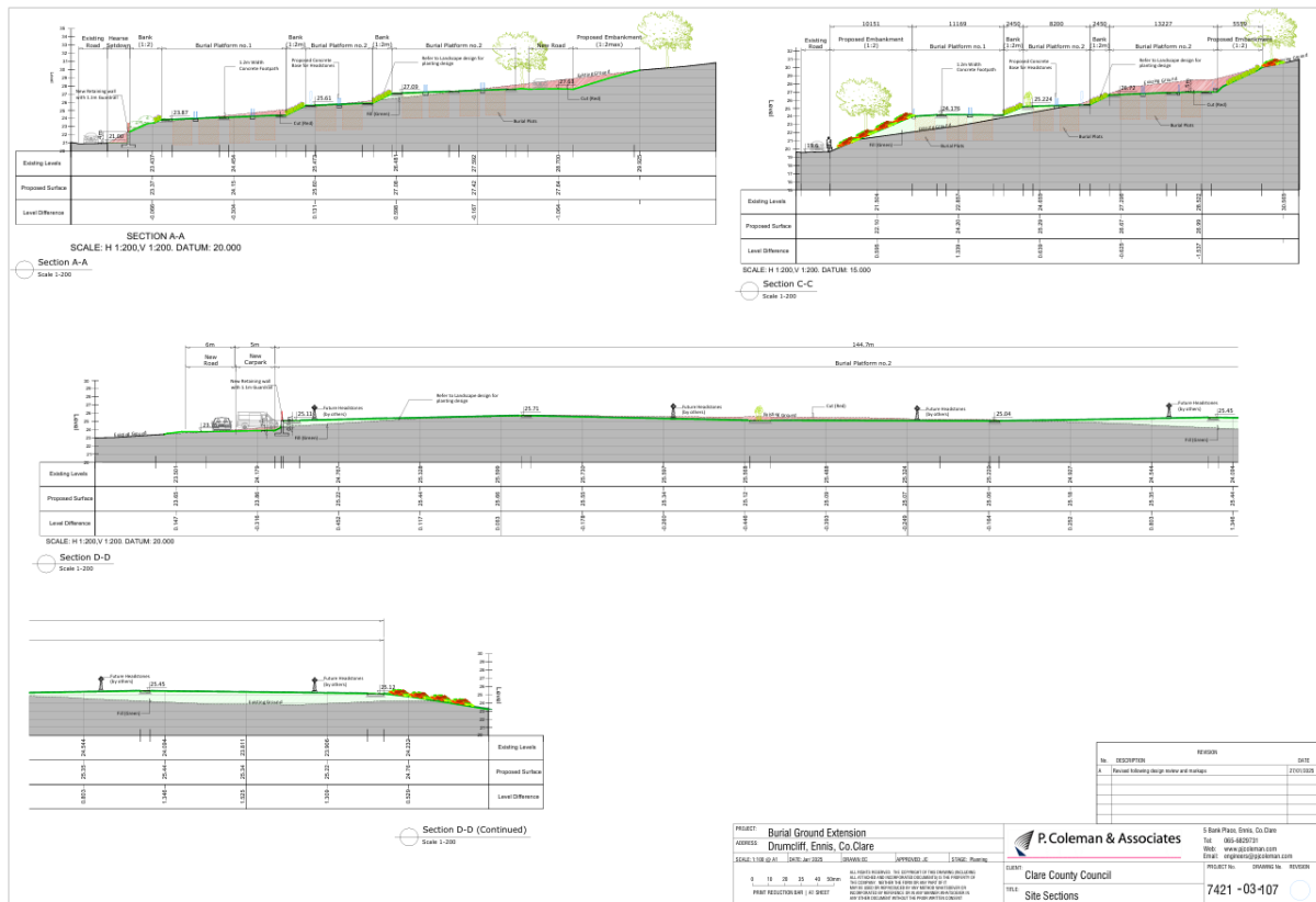
Figure I: Site Cross Section
