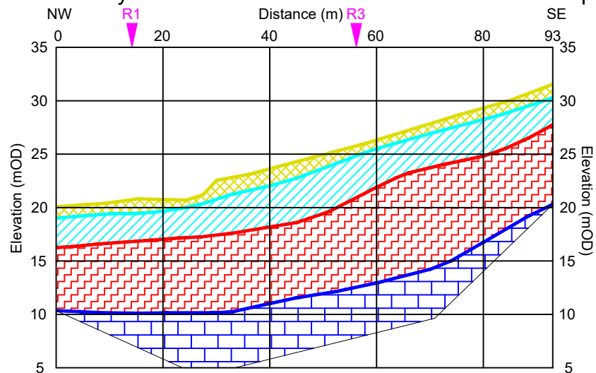
2D-Resistivity Line R2 and Seismic Refraction Line S2 Interpretation
