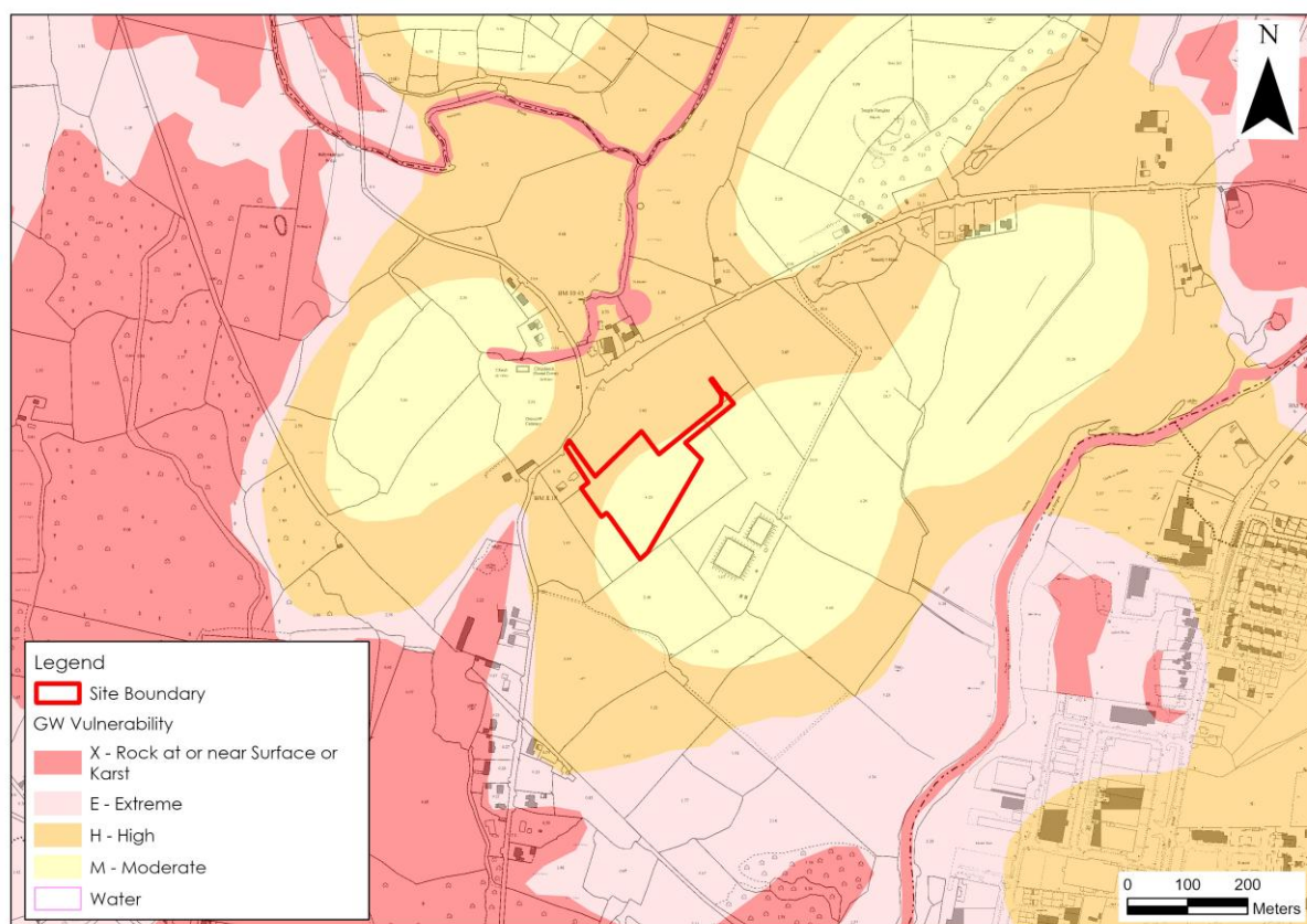
Figure E: Groundwater Vulnerability Map
