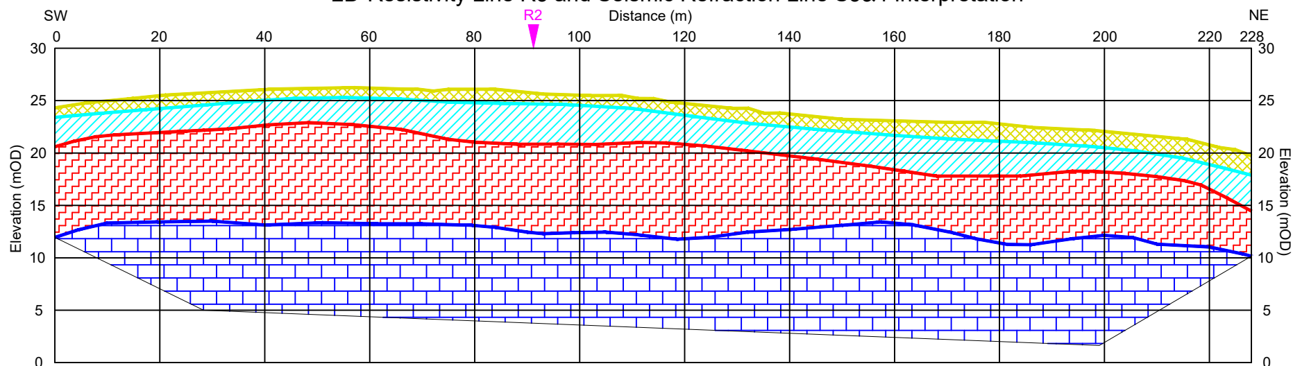
2D-Resistivity Line R3 and Seismic Refraction Line S3&4 Interpretation
