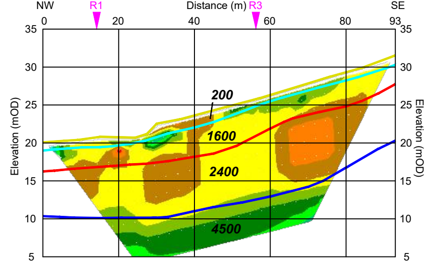
2D-Resistivity Line R2 and Seismic Refraction Line S2 Model
