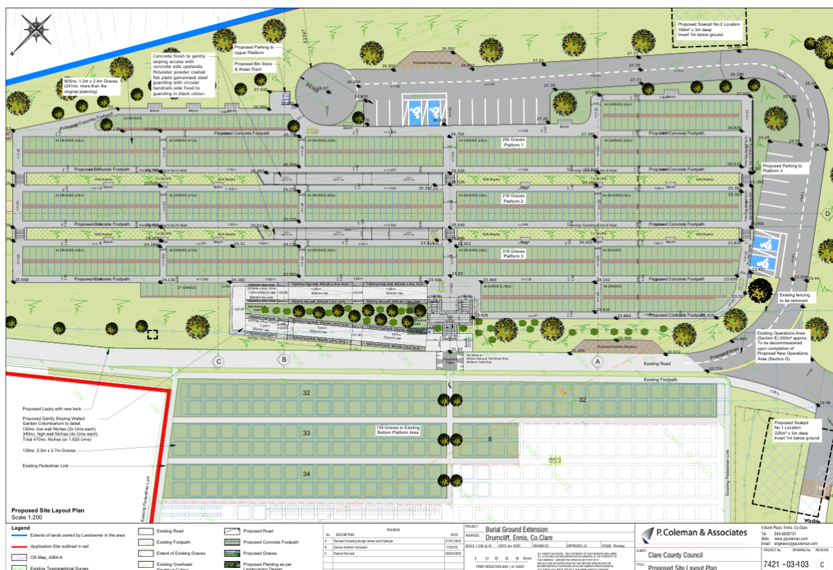
Figure H: Proposed Site Layout
