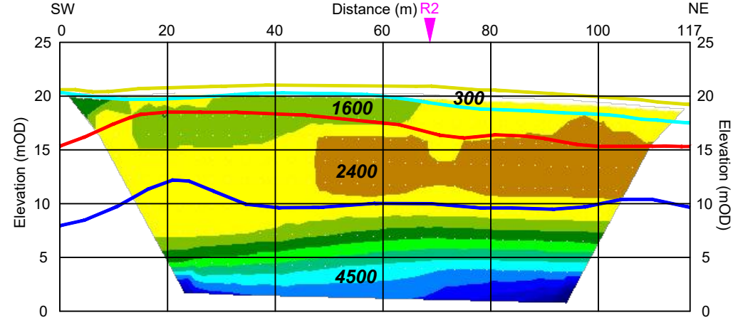
2D-Resistivity Line R1 and Seismic Refraction Line S1 Model
