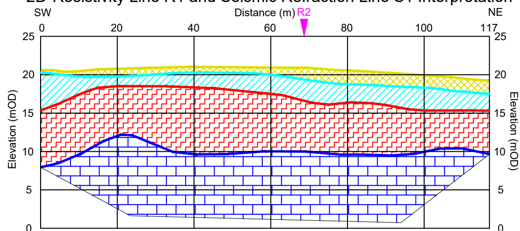
2D-Resistivity Line R1 and Seismic Refraction Line S1 Interpretation
